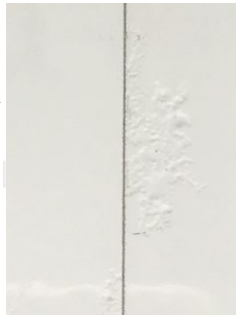
Corrosion morphology – Type B 腐蚀形貌 – 类型B
