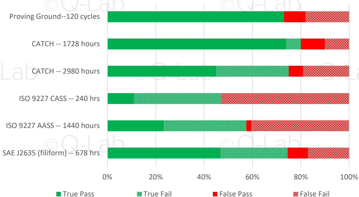
Pass/Fail Compared to Salt Accelerated Outdoor
